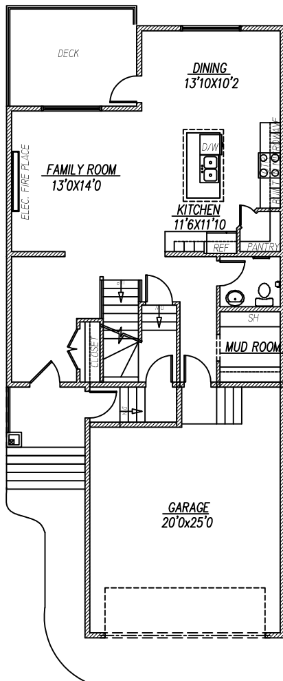
MAIN FLOOR PLAN 898 SQ.FT.
