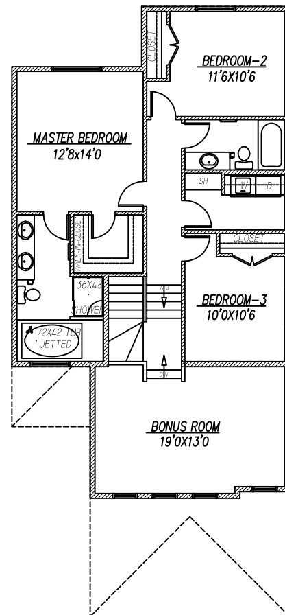
UPPER FLOOR PLAN 1184 SQ.FT.
