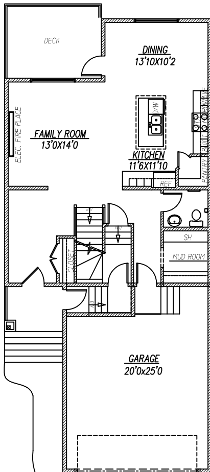
MAIN FLOOR PLAN 898 SQ.FT.
